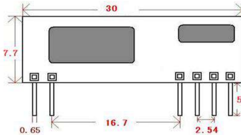
CY120 Dimension
