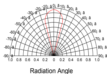
Radiation Characteristics
