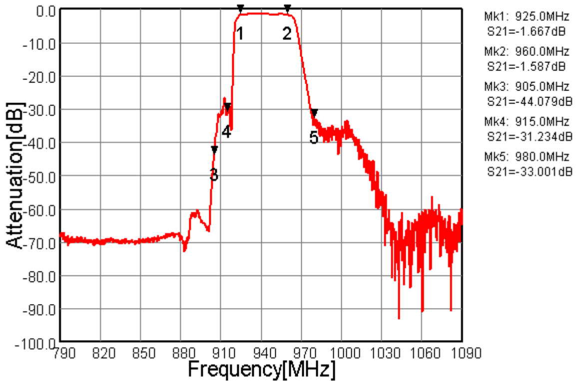
Pass-band Characteristics
