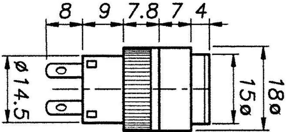
Outline Drawing
