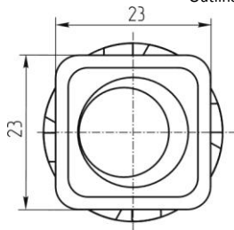
Outline Drawing
