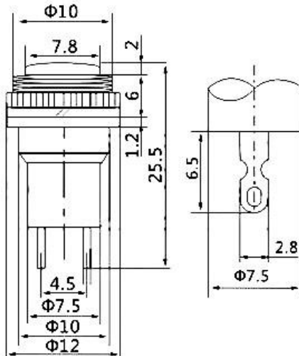
Outline Drawing
